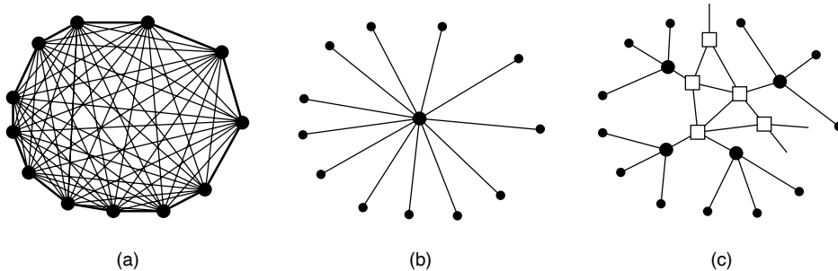
Figure 2-24. (a) Fully interconnected network. (b) Centralized switch. (c) Two-level hierarchy.
