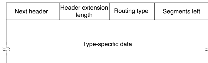
Figure 5-60. The extension header for routing.
