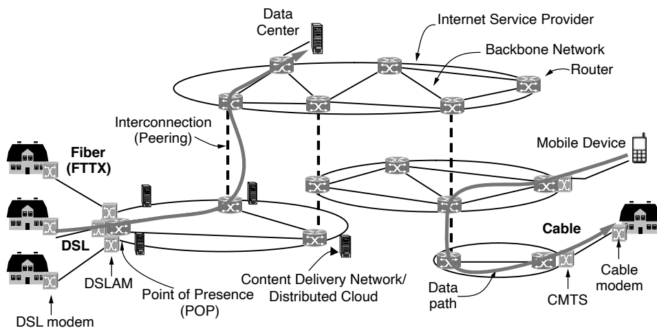
Figure 1-16. Overview of the Internet architecture.
