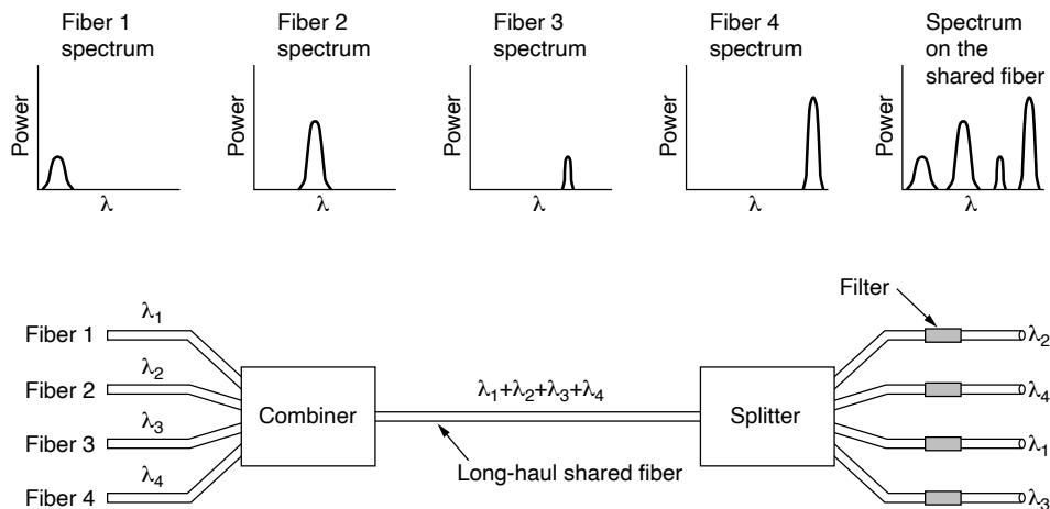
Figure 2-23. Wavelength division multiplexing.
