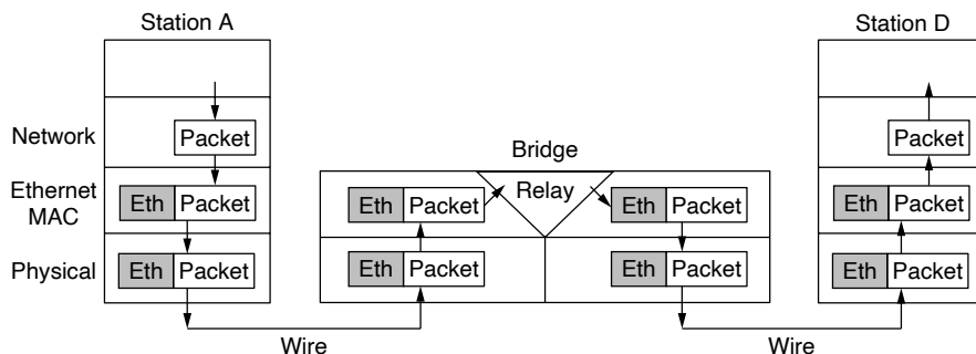
Figure 4-34. Protocol processing at a bridge.
