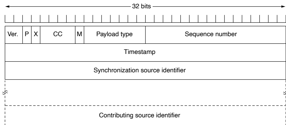
Figure 6-31. The RTP header.
