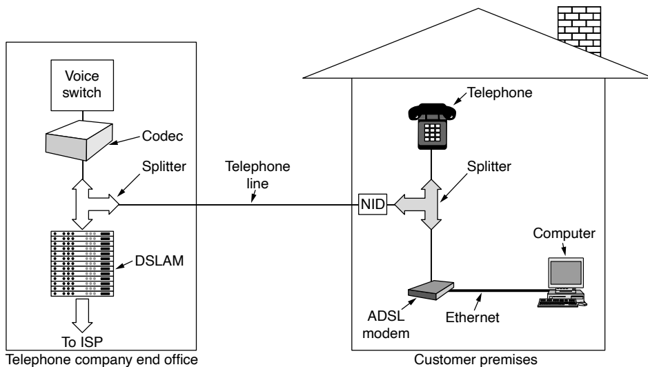
Figure 2-30. A typical ADSL equipment configuration.
