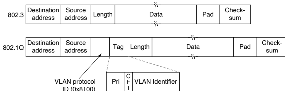
Figure 4-41. The 802.3 (legacy) and 802.1Q Ethernet frame formats.
