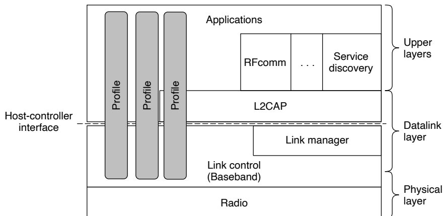
Figure 4-31. The Bluetooth protocol architecture.
