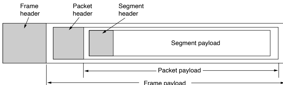
Figure 6-3. Nesting of segments, packets, and frames.
