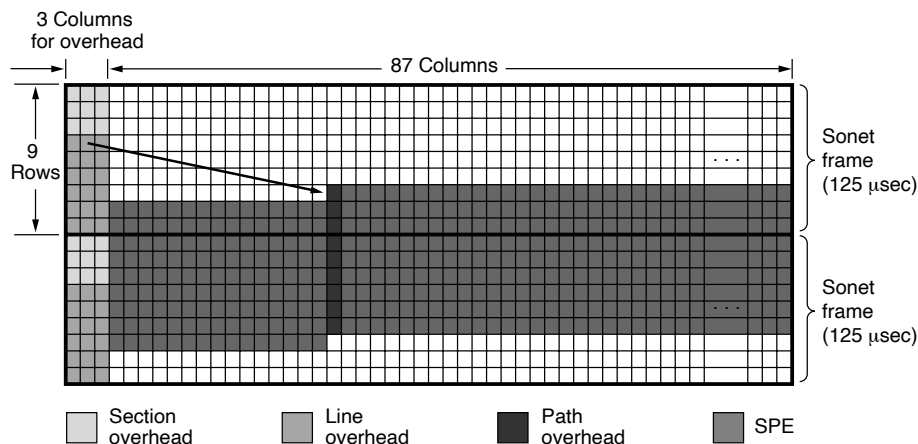
Figure 2-34. Two back-to-back SONET frames.
