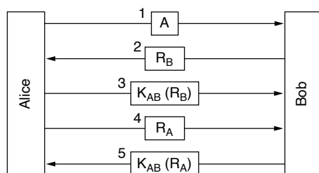
Figure 8-29. Two-way authentication using a challenge-response protocol.
