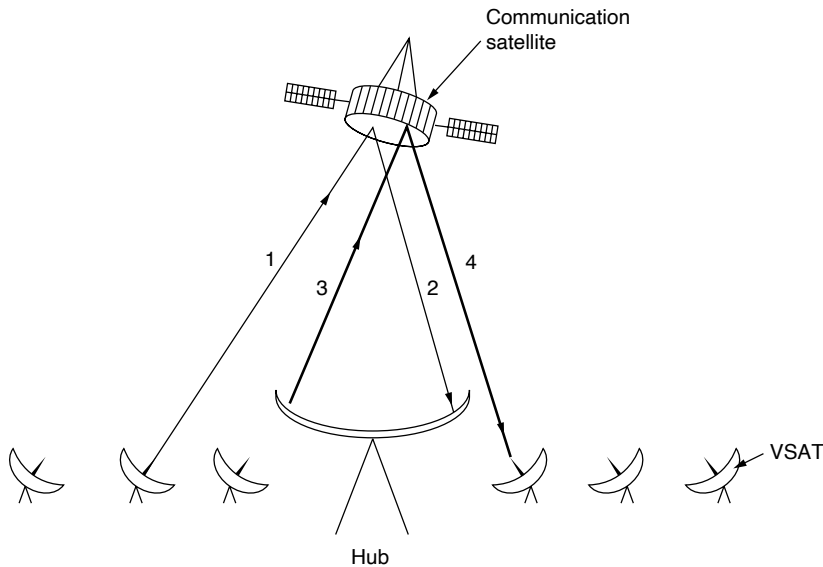
Figure 2-50. VSATs using a hub.
