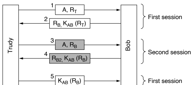
Figure 8-31. The reflection attack.
