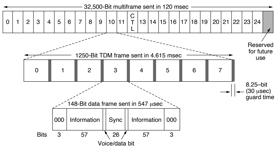
Figure 2-42. A portion of the GSM framing structure.
