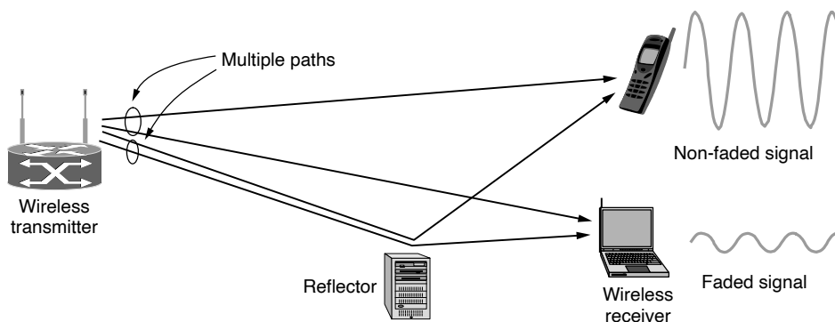
Figure 1-23. Multipath fading.
