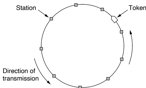
Figure 4-7. Token ring.
