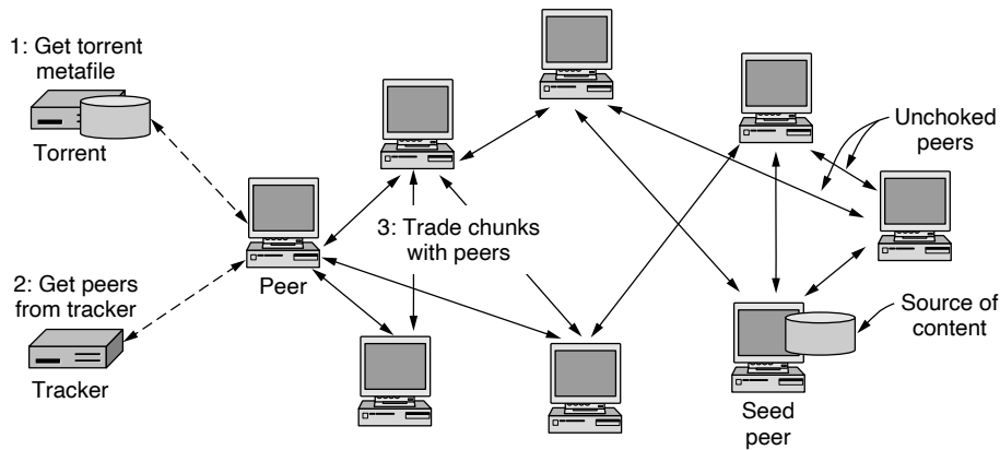
Figure 7-47. BitTorrent.
