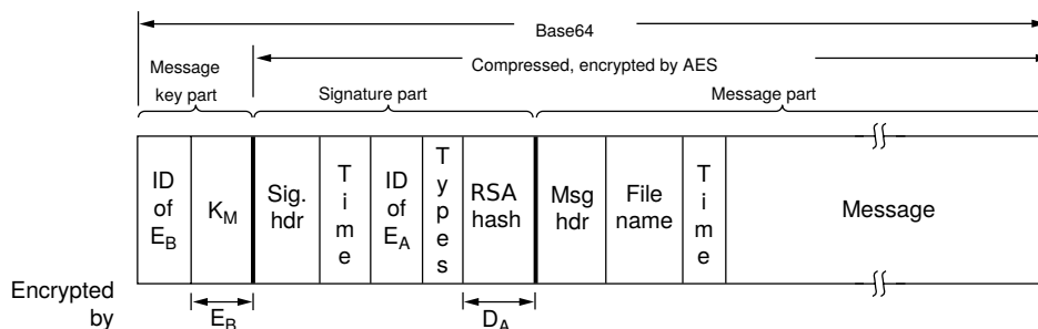
Figure 8-46. A PGP message.
