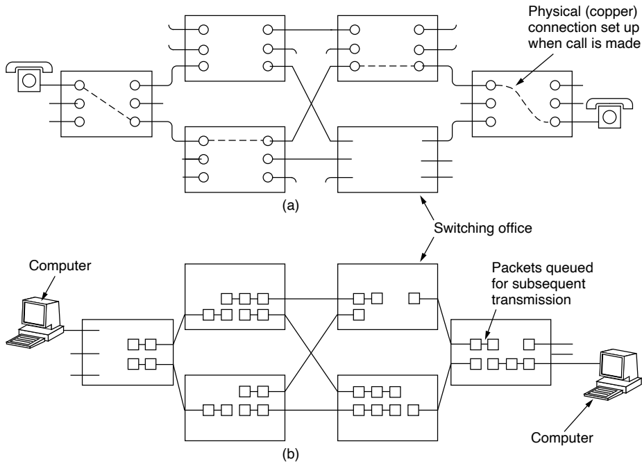
Figure 2-36. (a) Circuit switching. (b) Packet switching.
