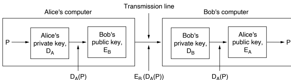
Figure 8-22. Digital signatures using public-key cryptography.
