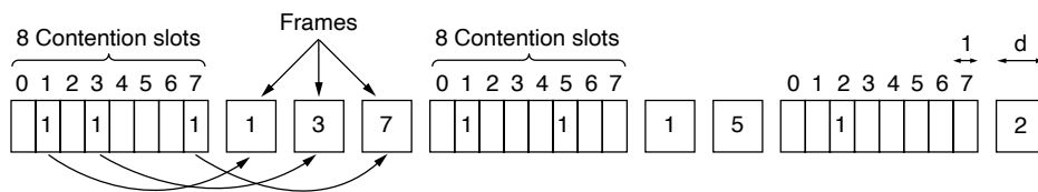
Figure 4-6. The basic bit-map protocol.
