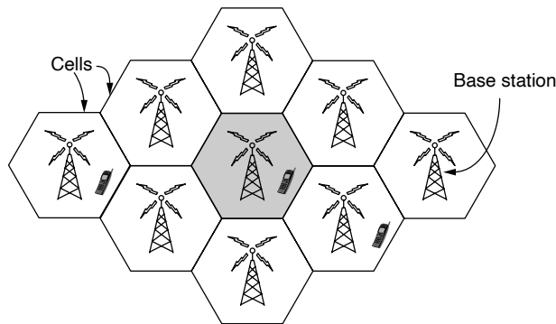
Figure 1-21. Cellular design of mobile phone networks.
