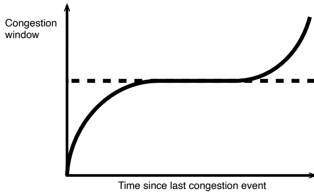
Figure 6-49. Evolution of TCP CUBIC Congestion Window.
