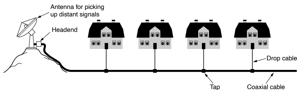
Figure 2-44. An early cable television system.
