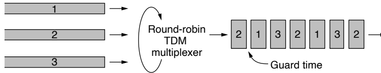
Figure 2-21. Time Division Multiplexing (TDM).
