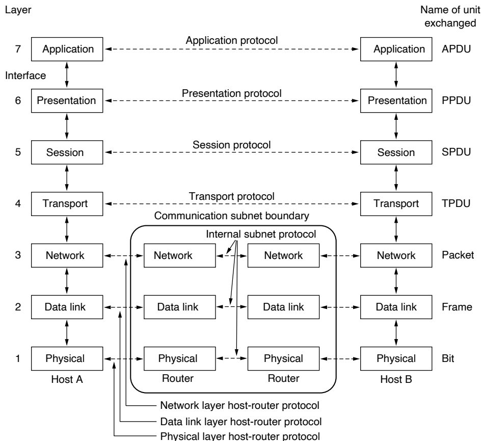
Figure 1-32. The OSI reference model.
