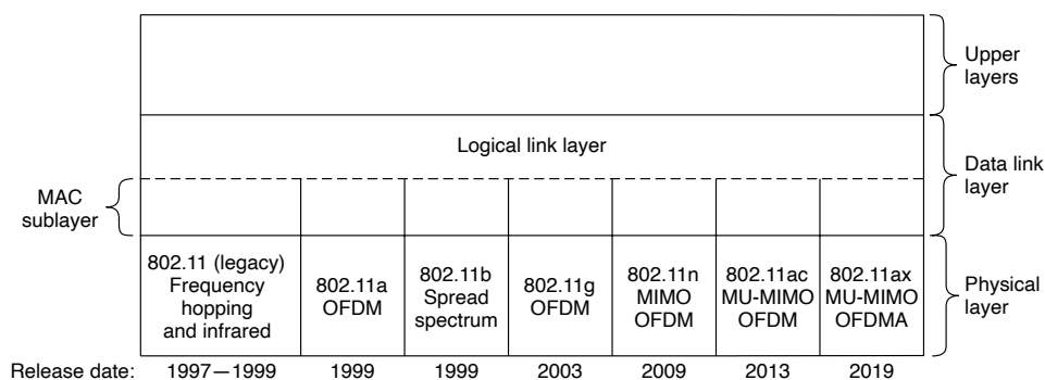
Figure 4-24. Part of the 802.11 protocol stack.
