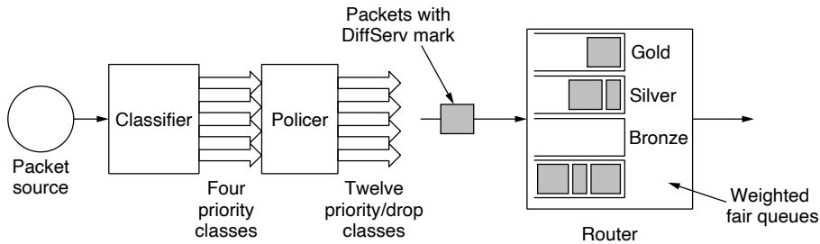
Figure 5-35. A possible implementation of assured forwarding.
