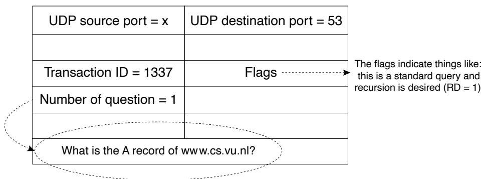
Figure 8-3. A DNS request for www.cs.vu.nl .
