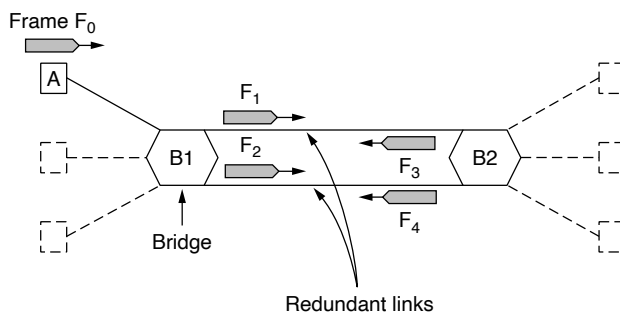
Figure 4-35. Bridges with two parallel links.
