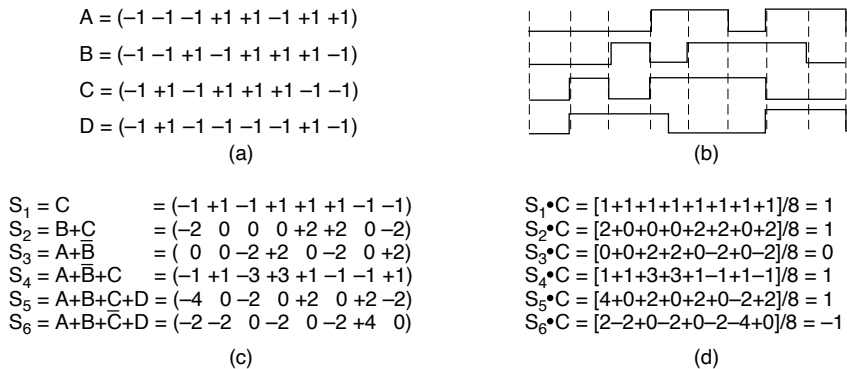
Figure 2-22. (a) Chip sequences for four stations. (b) Signals the sequences represent (c) Six examples of transmissions. (d) Recovery of station C's signal.
