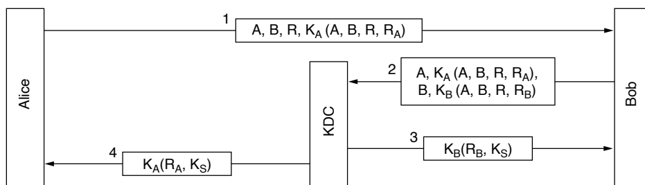
Figure 8-38. The Otway-Rees authentication protocol (slightly simplified).
