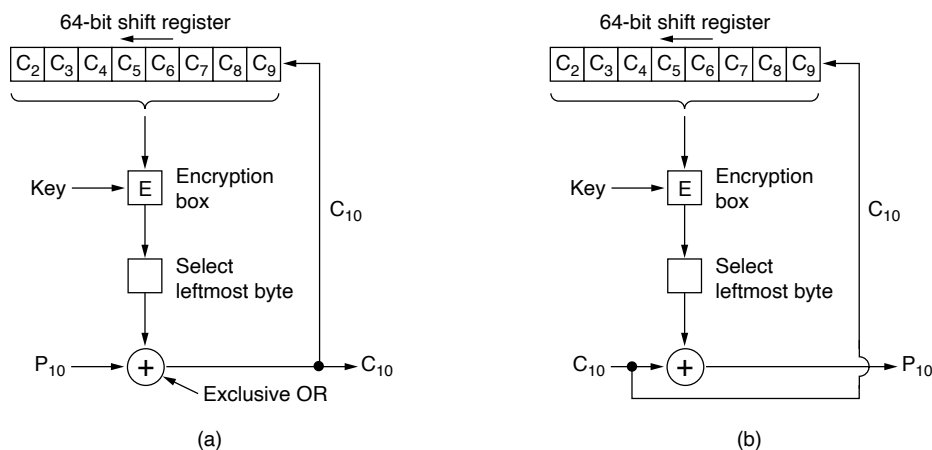
Figure 8-17. Cipher feedback mode. (a) Encryption. (b) Decryption.
