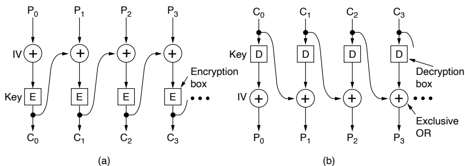
Figure 8-16. Cipher block chaining. (a) Encryption. (b) Decryption.
