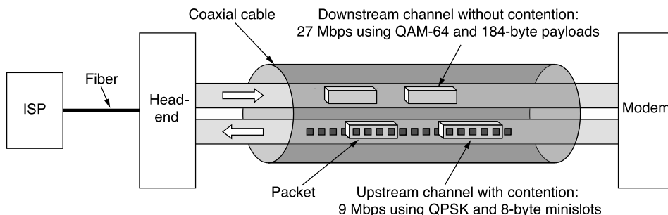
Figure 2-47. Typical details of the upstream and downstream channels in North America.
