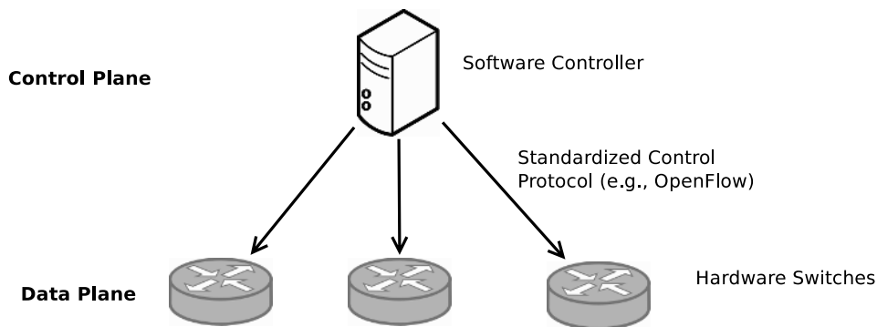
Figure 5-43. Control and data plane separation in SDN.
