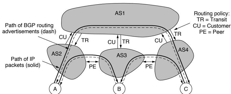
Figure 5-68. Routing policies between four autonomous systems.
