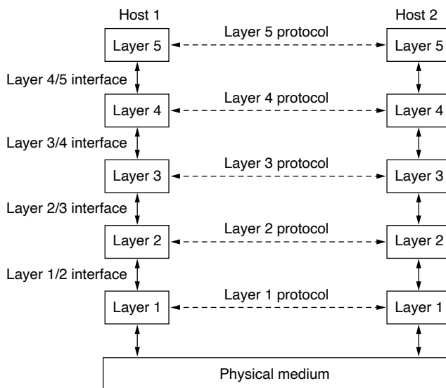
Figure 1-25. Layers, protocols, and interfaces.
