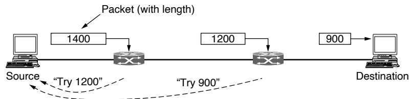
Figure 5-42. Path MTU discovery.
