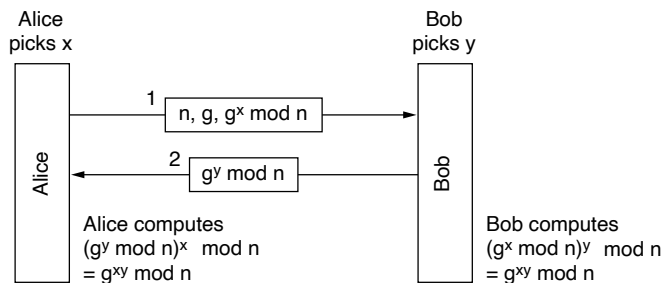
Figure 8-34. The Diffie-Hellman key exchange.
