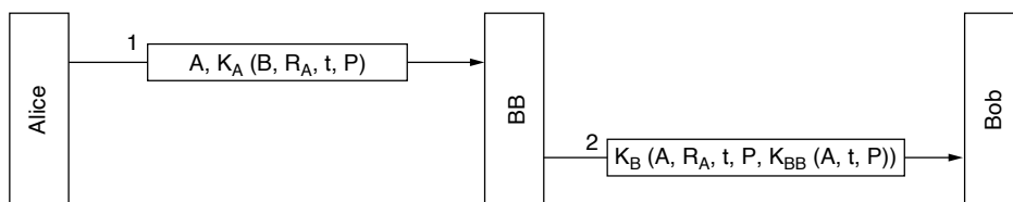
Figure 8-21. Digital signatures with Big Brother.
