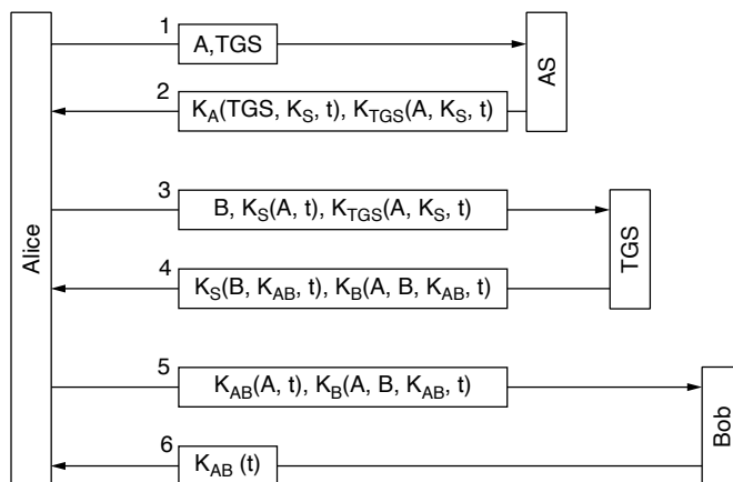
Figure 8-39. The operation of Kerberos V5.
