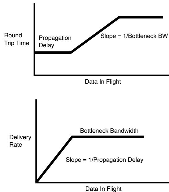
Figure 6-50. BBR Operating Point.
