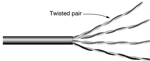
Figure 2-1. Category 5e UTP cable with four twisted pairs. These cables can be used for local area networks.
