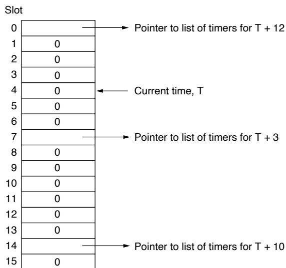
Figure 6-54. A timing wheel.
