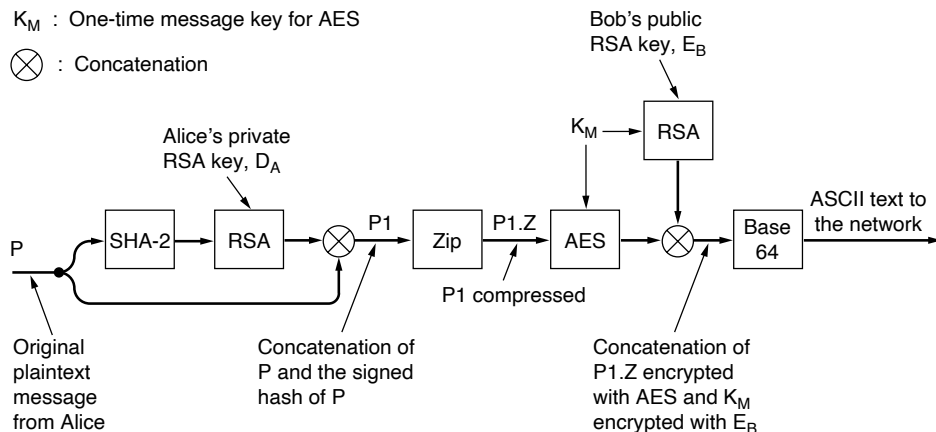
Figure 8-45. PGP in operation for sending a message.
