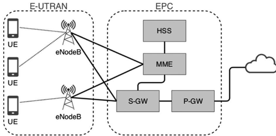
Figure 1-19. Simplified 4G LTE network architecture.
