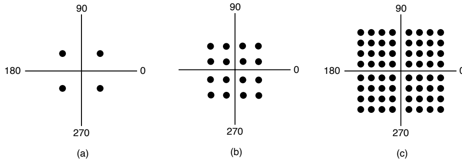
Figure 2-17. (a) QPSK. (b) QAM-16. (c) QAM-64.
