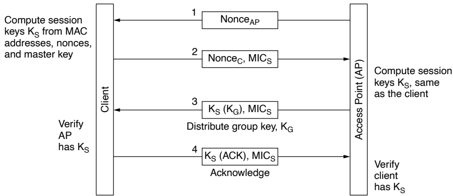
Figure 8-44. The 802.11i key setup handshake.
