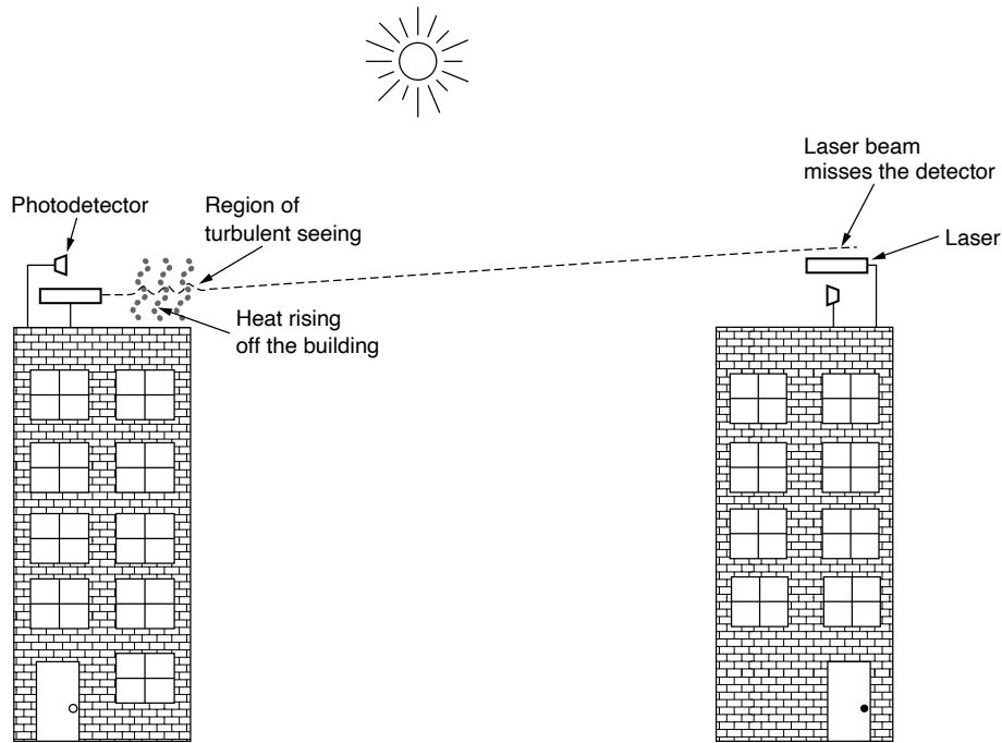
Figure 2-11. Convection currents can interfere with laser communication systems. A bidirectional system with two lasers is pictured here.
