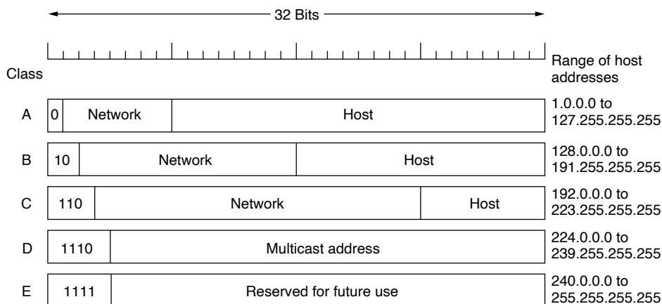
Figure 5-54. IP address formats.
