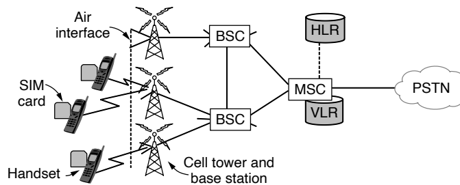
Figure 2-40. GSM mobile network architecture.
