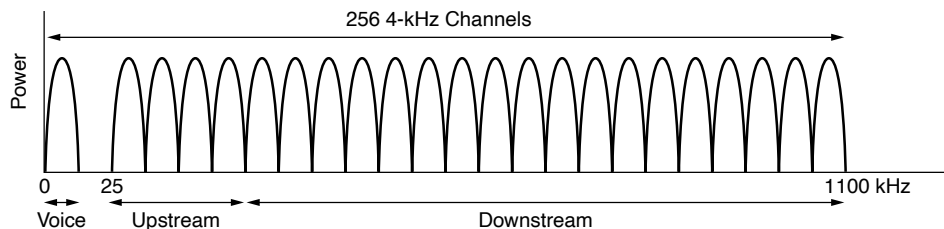
Figure 2-29. Operation of ADSL using discrete multitone modulation.
