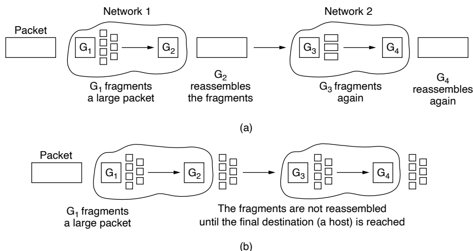
Figure 5-40. (a) Transparent fragmentation. (b) Nontransparent fragmentation.
