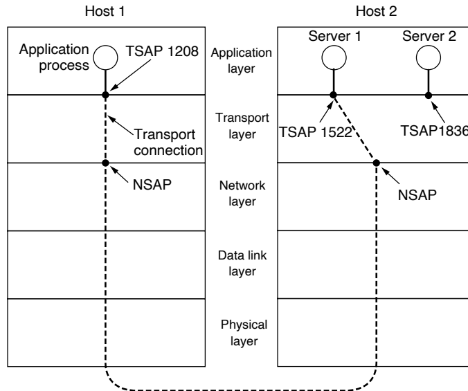
Figure 6-8. TSAPs, NSAPs, and transport connections.
