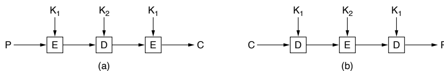
Figure 8-14. (a) Triple encryption using DES. (b) Decryption.
