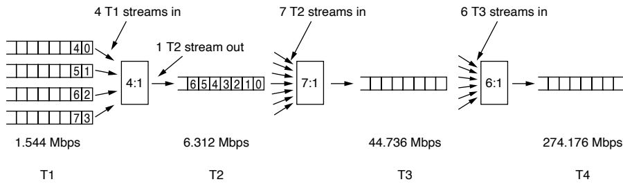
Figure 2-33. Multiplexing T1 streams into higher carriers.
