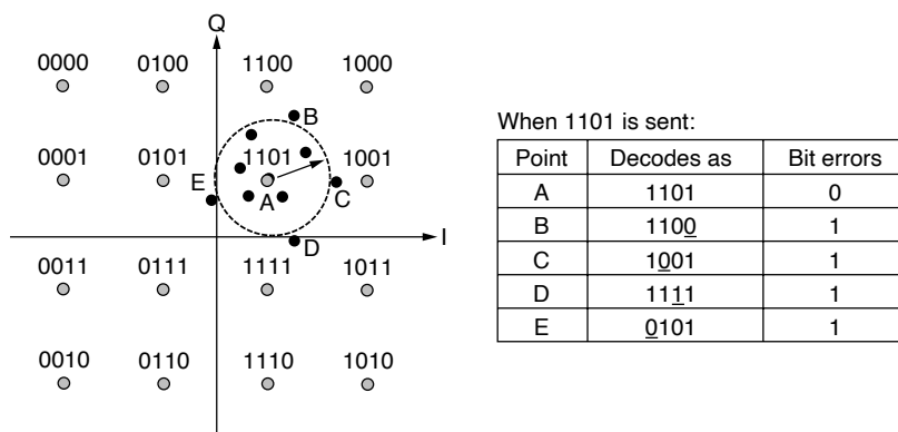
Figure 2-18. Gray-coded QAM-16.
