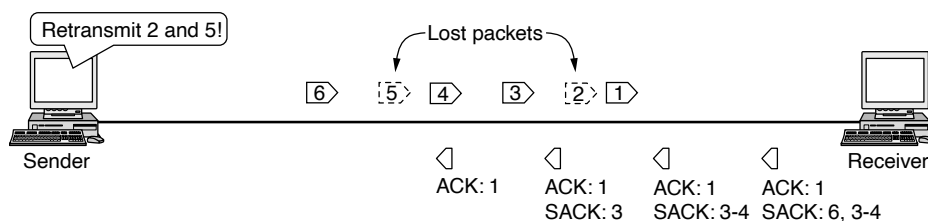
Figure 6-48. Selective acknowledgements.
