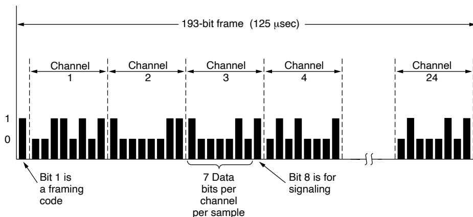
Figure 2-32. The T1 carrier (1.544 Mbps).
