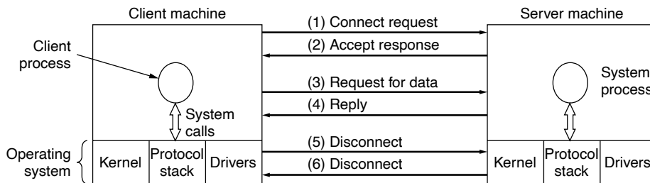
Figure 1-30. A simple client-server interaction using acknowledged datagrams.
