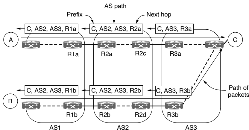
Figure 5-69. Propagation of BGP route advertisements.
