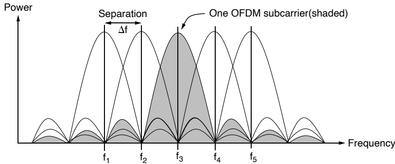
Figure 2-20. Orthogonal frequency division multiplexing (OFDM).
