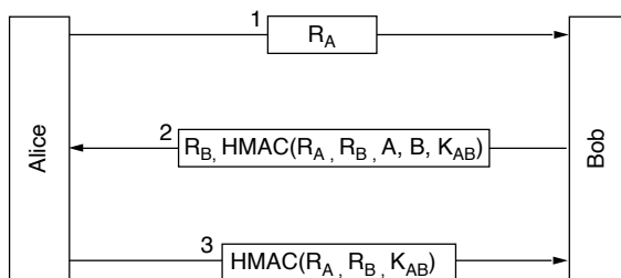
Figure 8-33. Authentication using HMACs.
