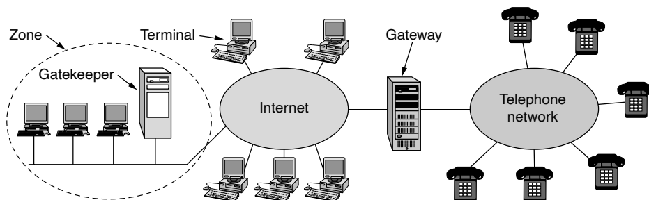
Figure 7-36. The H.323 architectural model for Internet telephony.
