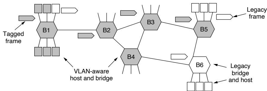
Figure 4-40. Bridged LAN that is only partly VLAN aware. The shaded symbols are VLAN aware. The empty ones are not.
