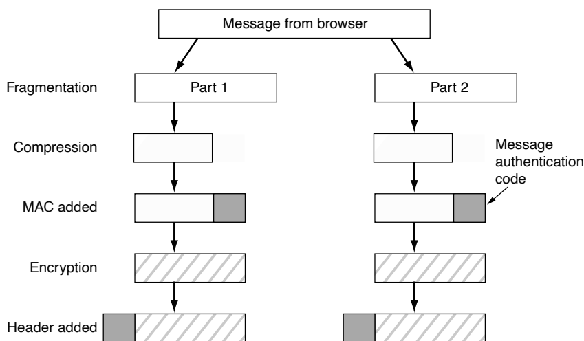
Figure 8-50. Data transmission using SSL.
