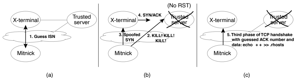
Figure 8-6. Mitnick's attack
