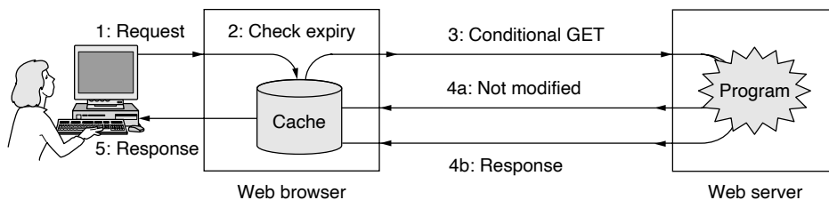
Figure 7-28. HTTP caching.
