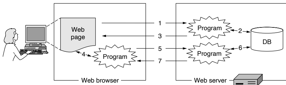
Figure 7-23. Dynamic pages.
