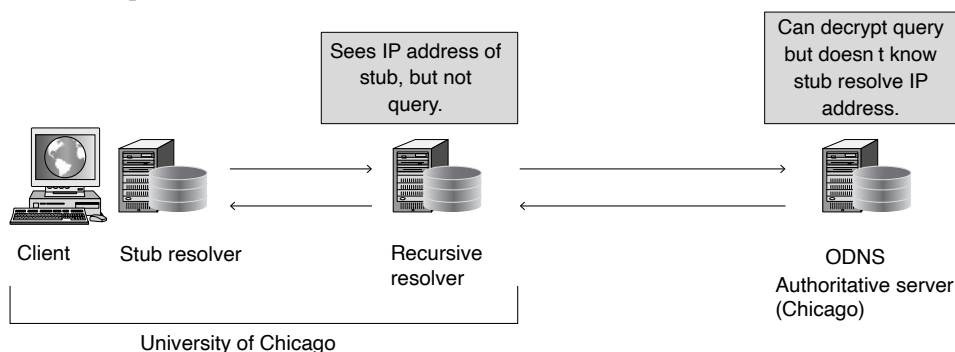
Figure 7-8. Oblivious DNS.
