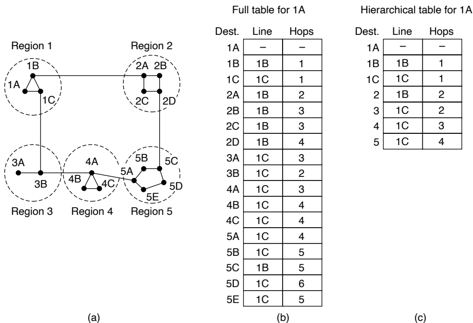
Figure 5-14. Hierarchical routing.
