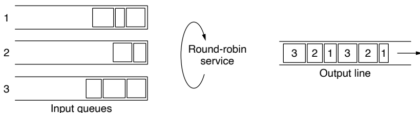
Figure 5-28. Round-robin fair queueing.
