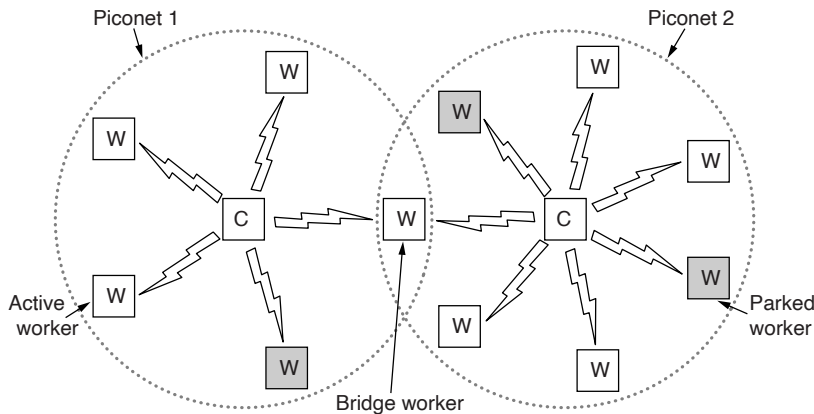
Figure 4-30. Two piconets can be connected to form a scatternet.
