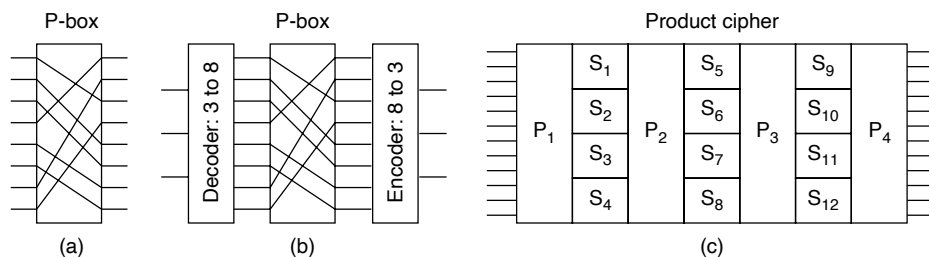
Figure 8-13. Basic elements of product ciphers. (a) P-box. (b) S-box. (c) Product.
