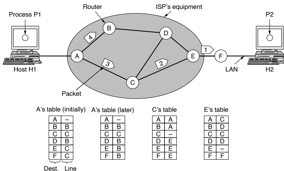
Figure 5-2. Routing within a datagram network.
