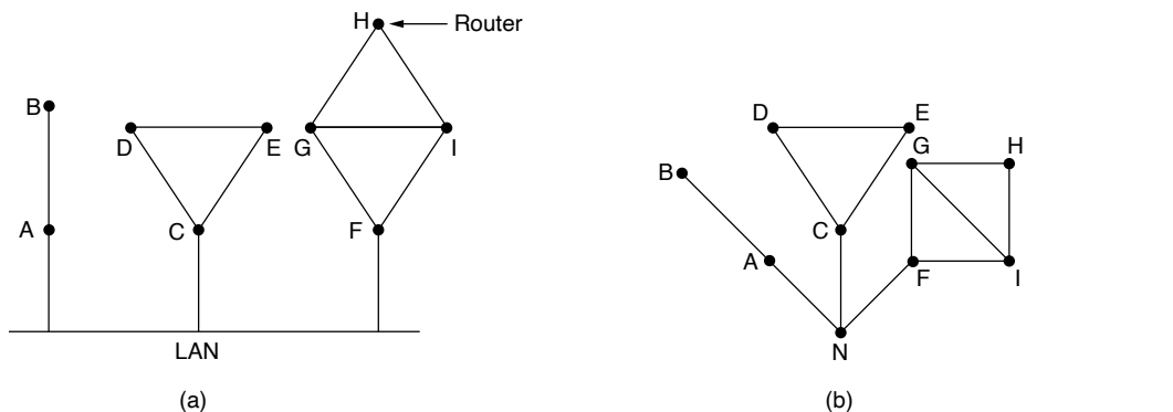
Figure 5-11. (a) Nine routers and a broadcast LAN. (b) A graph model of (a).
